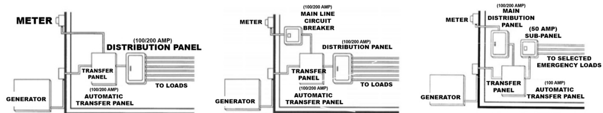
Typical service entrance ATS model installation (100/200A)
